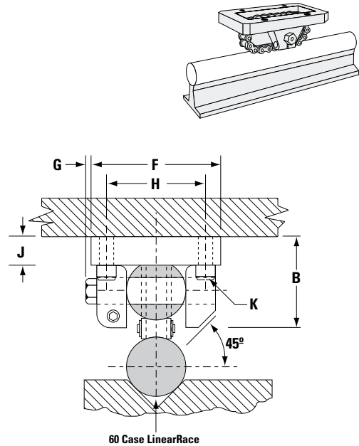
RoundWay Linear Roller Bearing (Single Type) and 60 Case LinearRace (Dimensions in inches)
