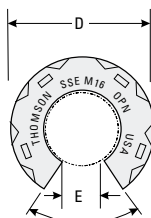
Super Smart Ball Bushing Bearings (Open Type) (Dimensions in mm)
